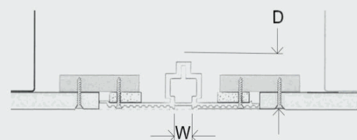
Section diagram of installed light fixture
